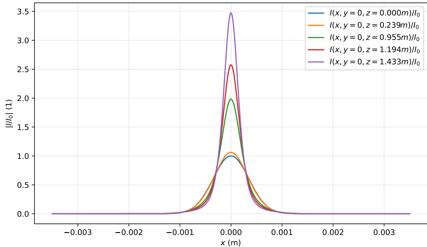
Intensity profile I(x, y = 0, z)/I_0 , \text{Pin}=1.3\text{Pcr} , artificial time
